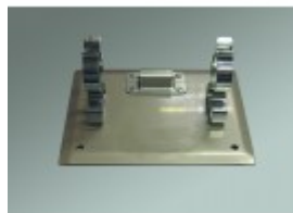
Bracket for multipurpose branchpipe, made of stainless steel, c/w 1 bracket holder for coupling key
