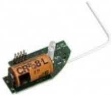
RadioLink module Ei600MRF, Lithium 3V 10 years battery Kurzbeschreibung Learn More
